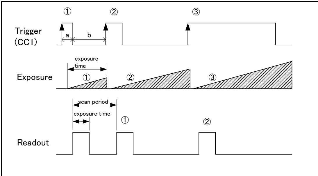
Figure 4-8-2-1 External Trigger Exposure Mode
