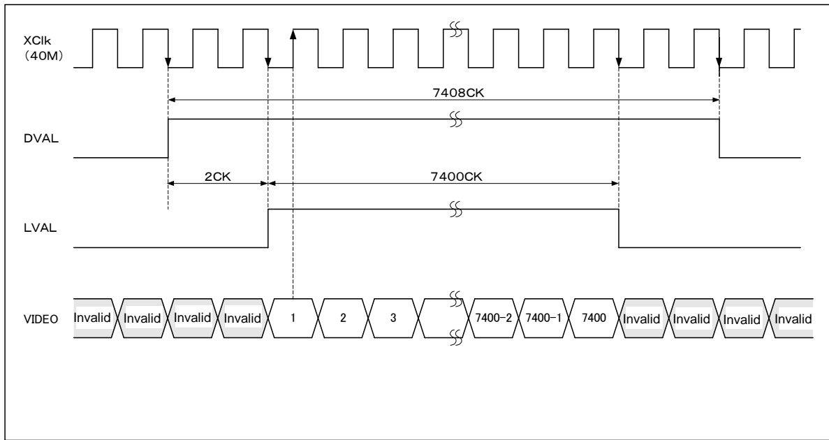
Figure 4-7-2 Video Output Phase
