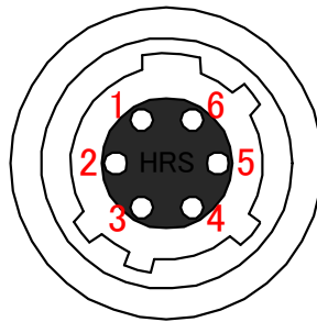
Figure 5-1-1 Pin Assignment of Power Cable
