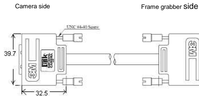
Figure 5-1-2 Connection Direction of Camera Cable
