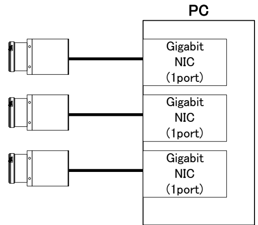
Example of connection between 1 PC and 3 cameras
