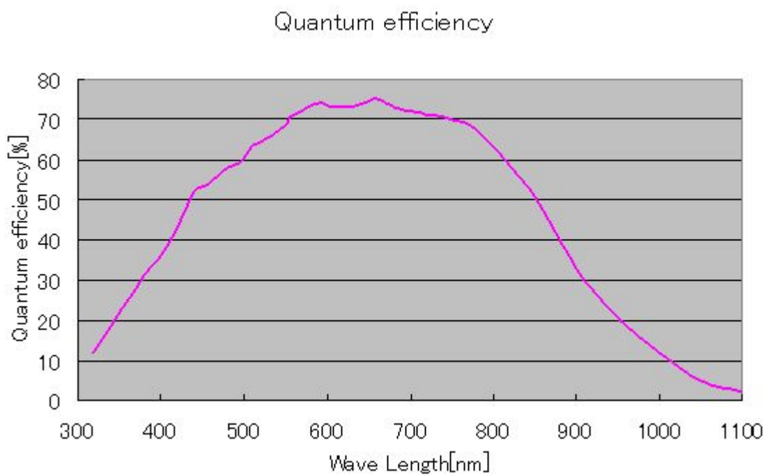
Figure 1-3-1 Spectral Responsivity
