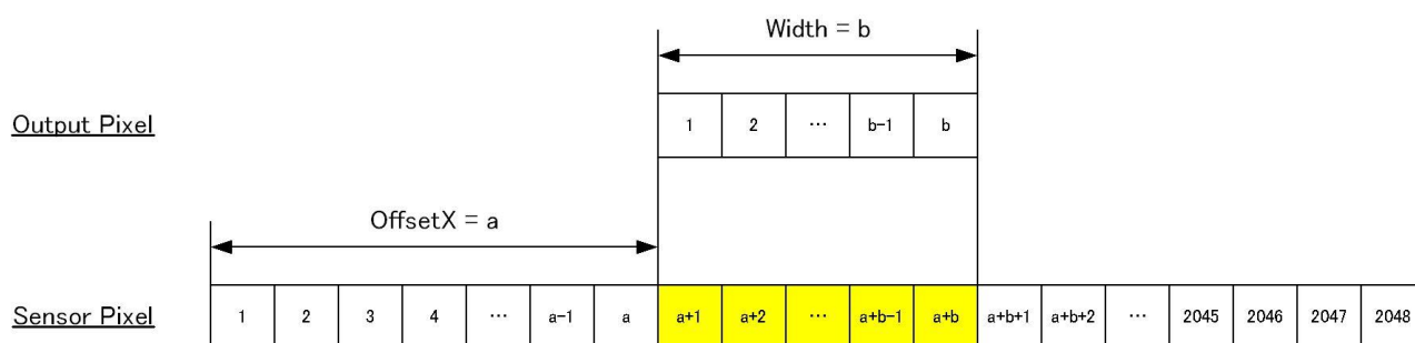
Figure 4-2-3-1 Valid Pixel Region
