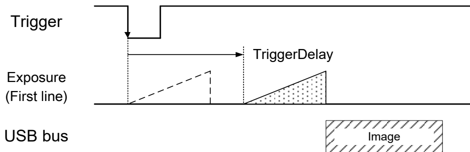
Trigger Delay
